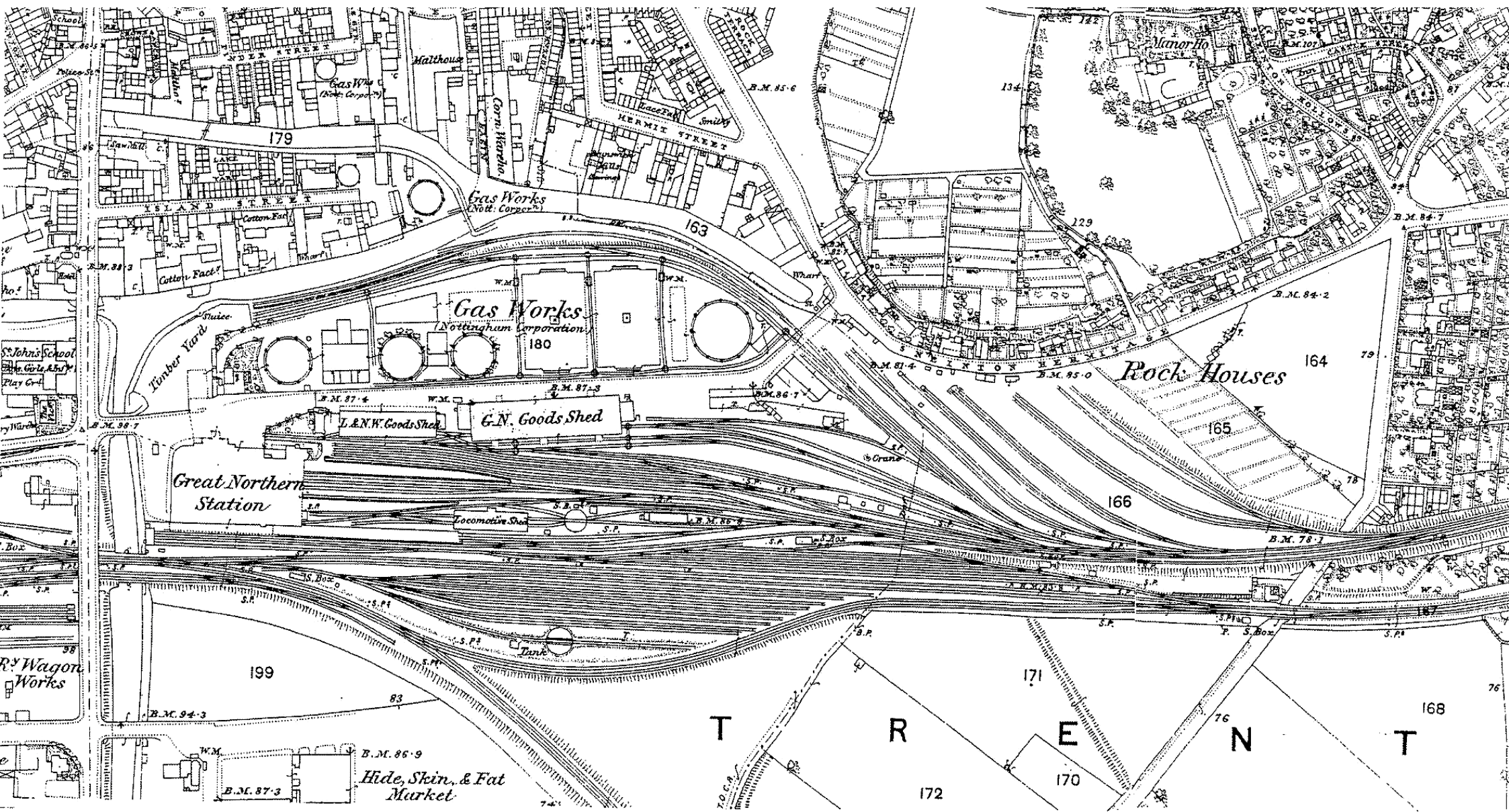
London Road Great Northern Station in 1881, showing its proximity to Sneinton. The Old Coal-yard sidings, where the collision took place, lie south of the signal box in the middle of the map. There may have been alterations to the layout between the date of the accident and the publication of this map.
